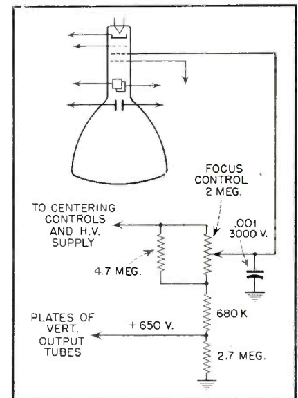
Fig. 4. Belmont focus network.
