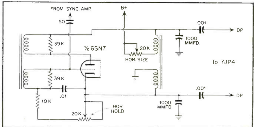
Admiral Model 19A1 - Partial schematic of hor. defl. circuit.
