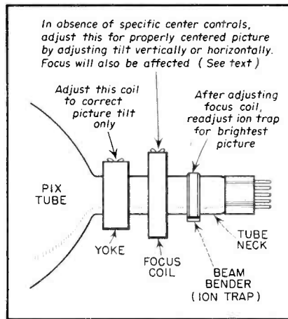
Fig. 3. Focus coil adjustment without centering controls.
