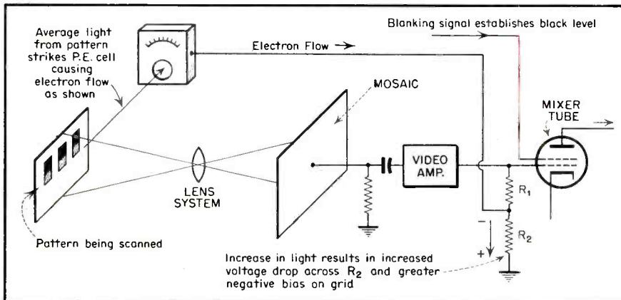
Fig. 1-20: Method of inserting average background brightness information of scene into video signal electrically. Complete video signal applied to mixer tube is voltage across R_1 + R_2 .
