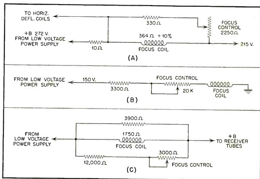
Fig. 2. Typical focus control circuits found in TV.
