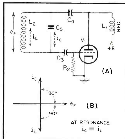
Fig. 1. Oscillator Circuit
